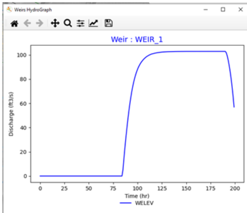
Figure 8.17 – Weirs HydroGraph
