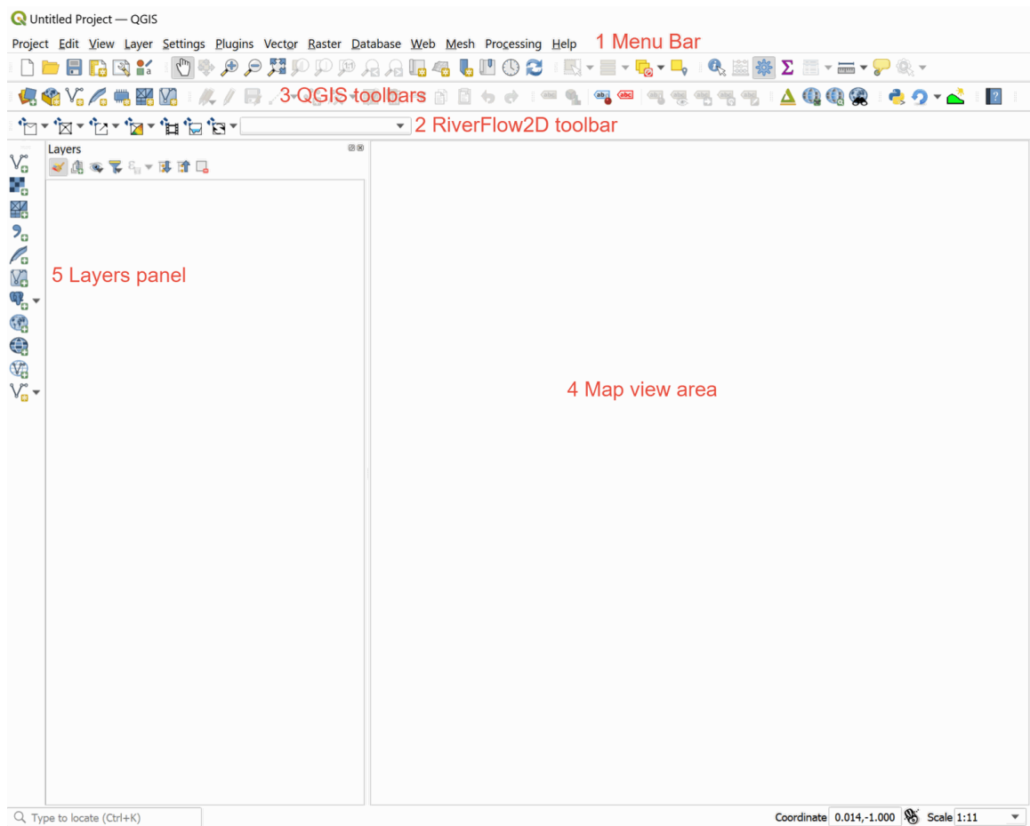
Figure 2.2 – QGIS interface indicating window areas.
